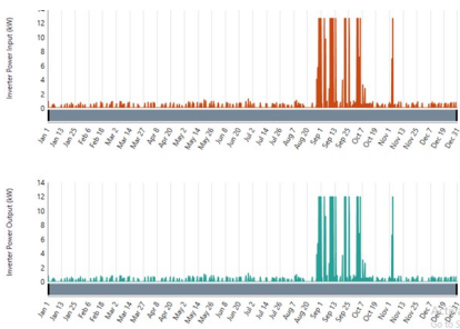
Figure 13: DC-AC converter operating hours per year
