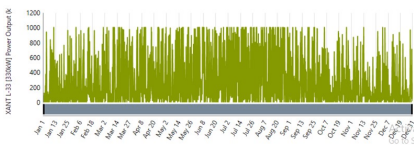
Figure 11: Power generation rate by wind turbine per day
